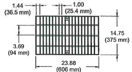
Galvanized Steel Grate Detail
