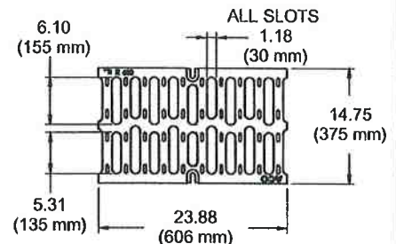
Ductile Iron Grate Detail
